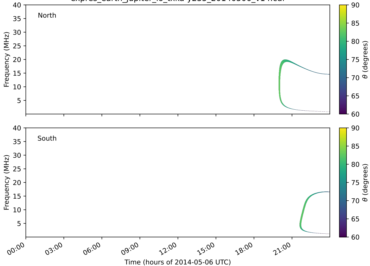
expres_earth_jupiter_io_txka-y235_20140506_v14.cdf
