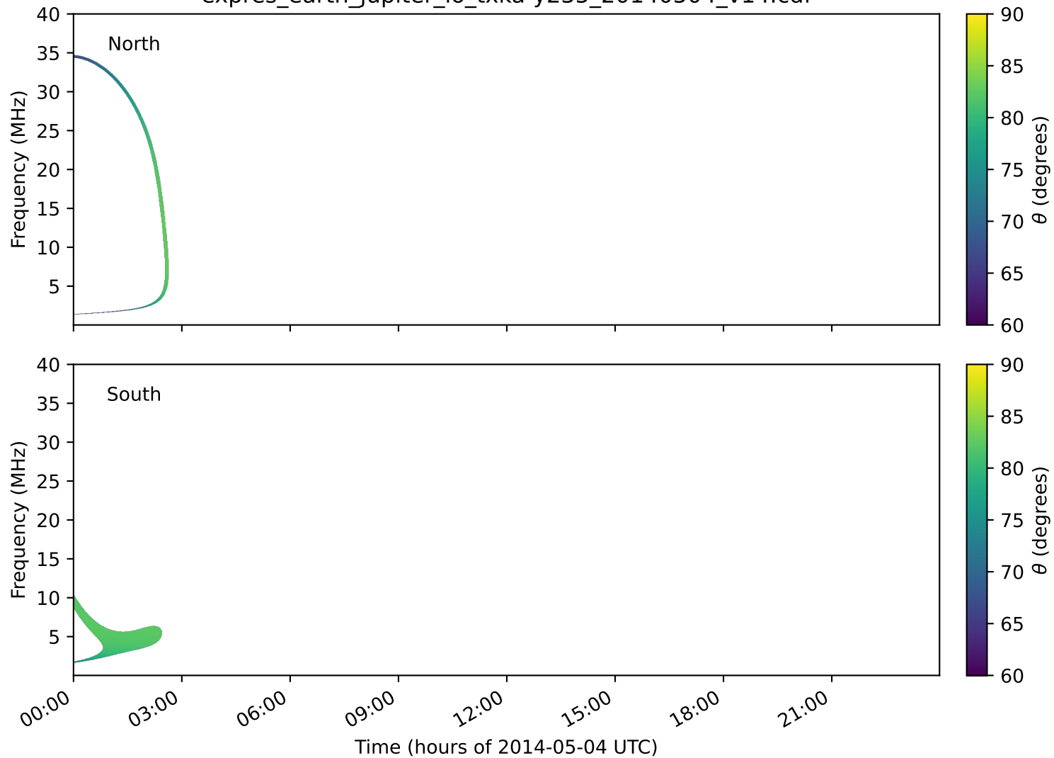
expres_earth_jupiter_io_txka-y235_20140504_v14.cdf
