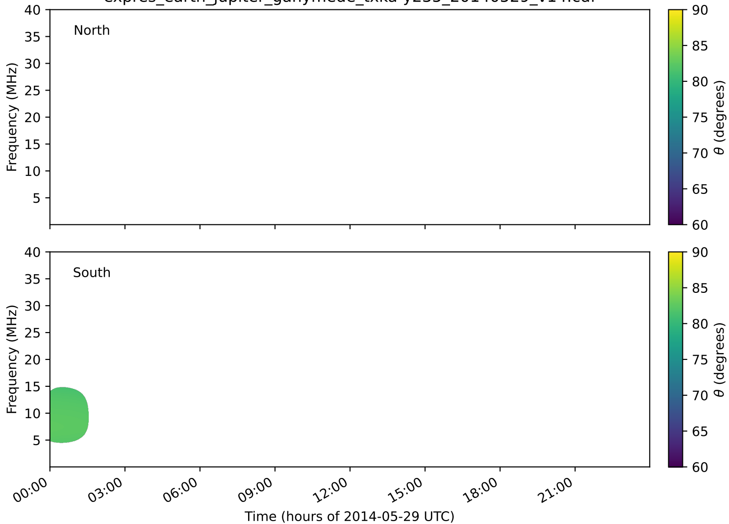
expres_earth_jupiter_ganymede_txka-y235_20140529_v14.cdf
