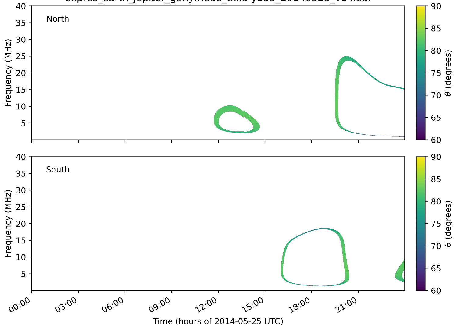
expres_earth_jupiter_ganymede_txka-y235_20140525_v14.cdf
