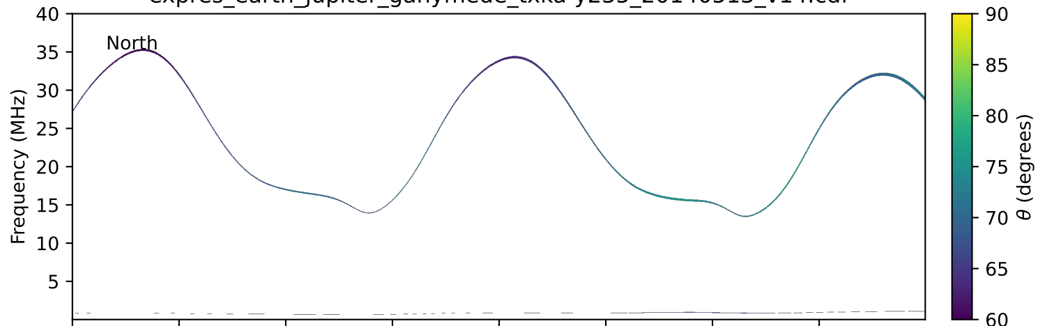
expres_earth_jupiter_ganymede_txka-y235_20140513_v14.cdf
