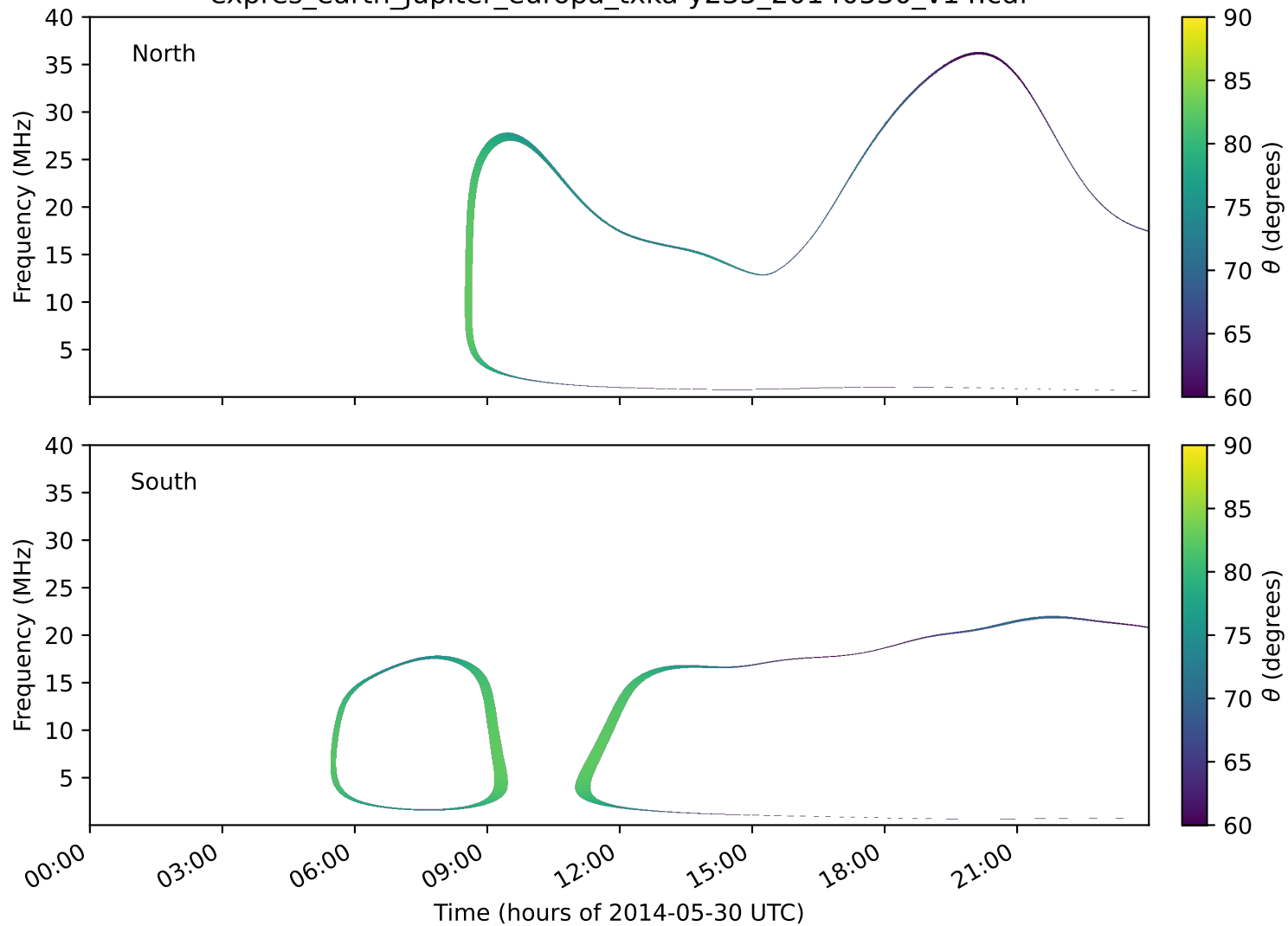
expres_earth_jupiter_europa_txka-y235_20140530_v14.cdf
