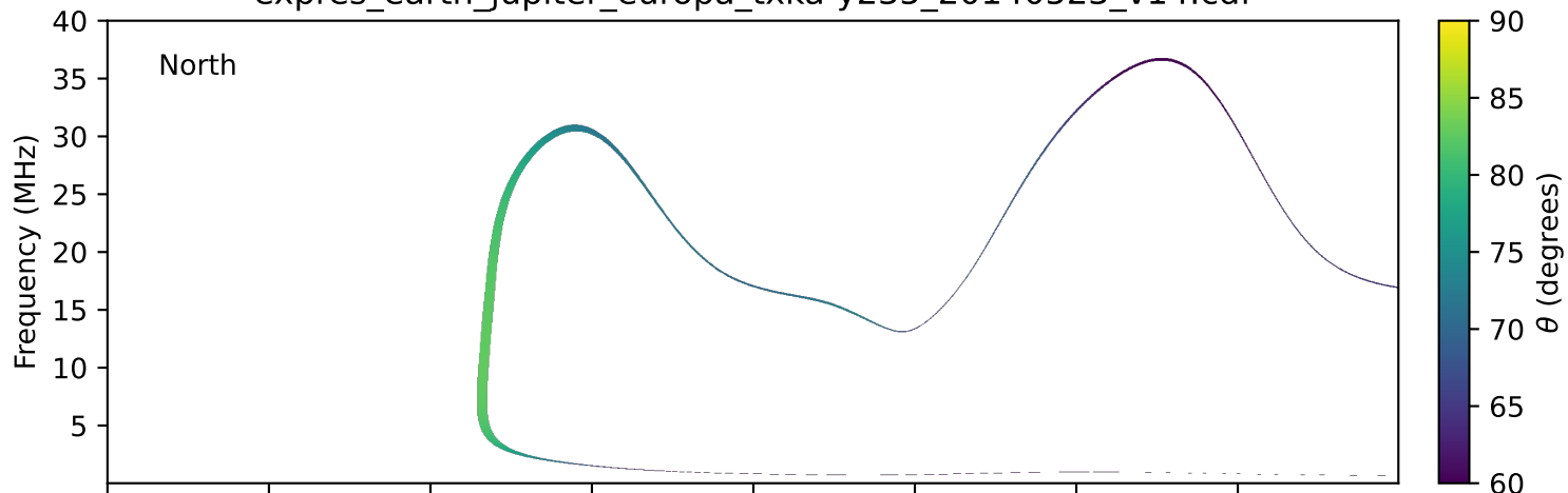
expres_earth_jupiter_europa_txka-y235_20140523_v14.cdf
