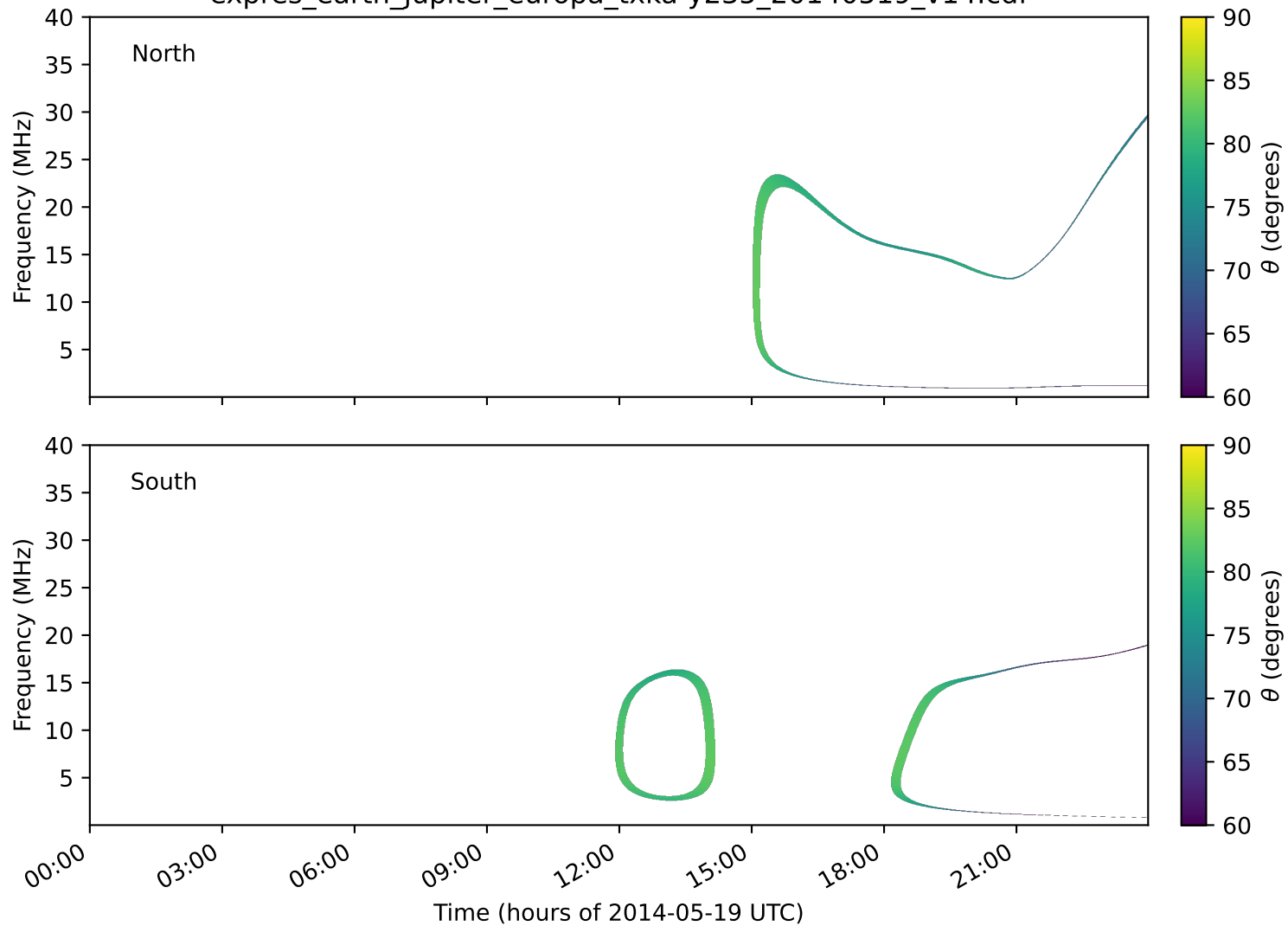
expres_earth_jupiter_europa_txka-y235_20140519_v14.cdf
