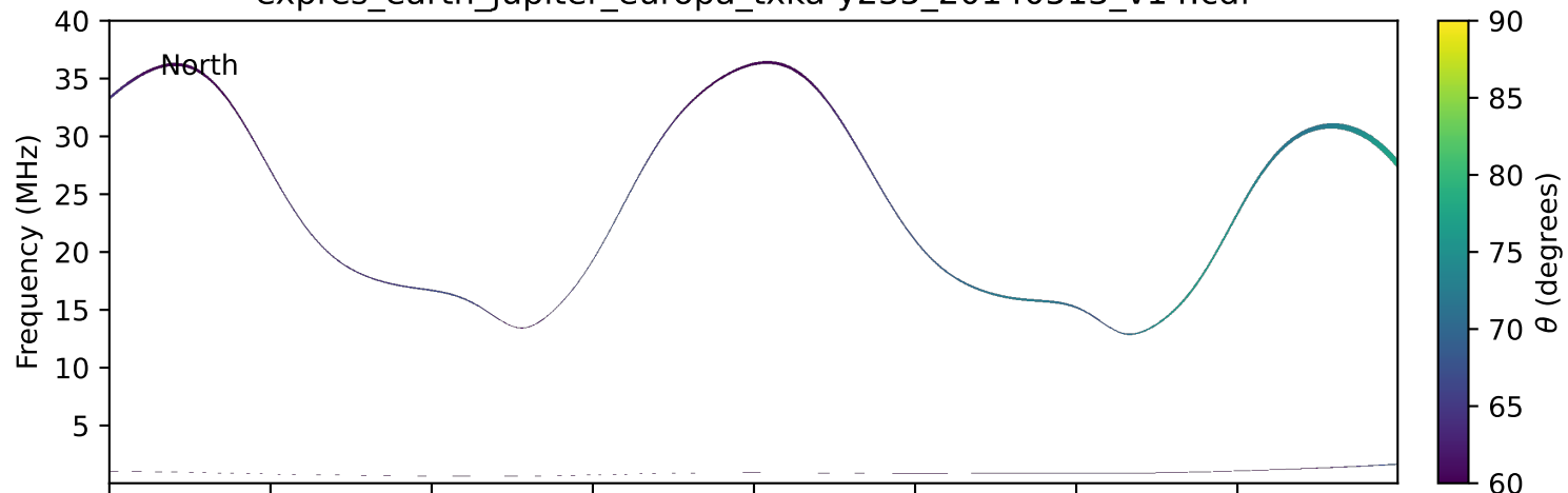
expres_earth_jupiter_europa_txka-y235_20140513_v14.cdf
