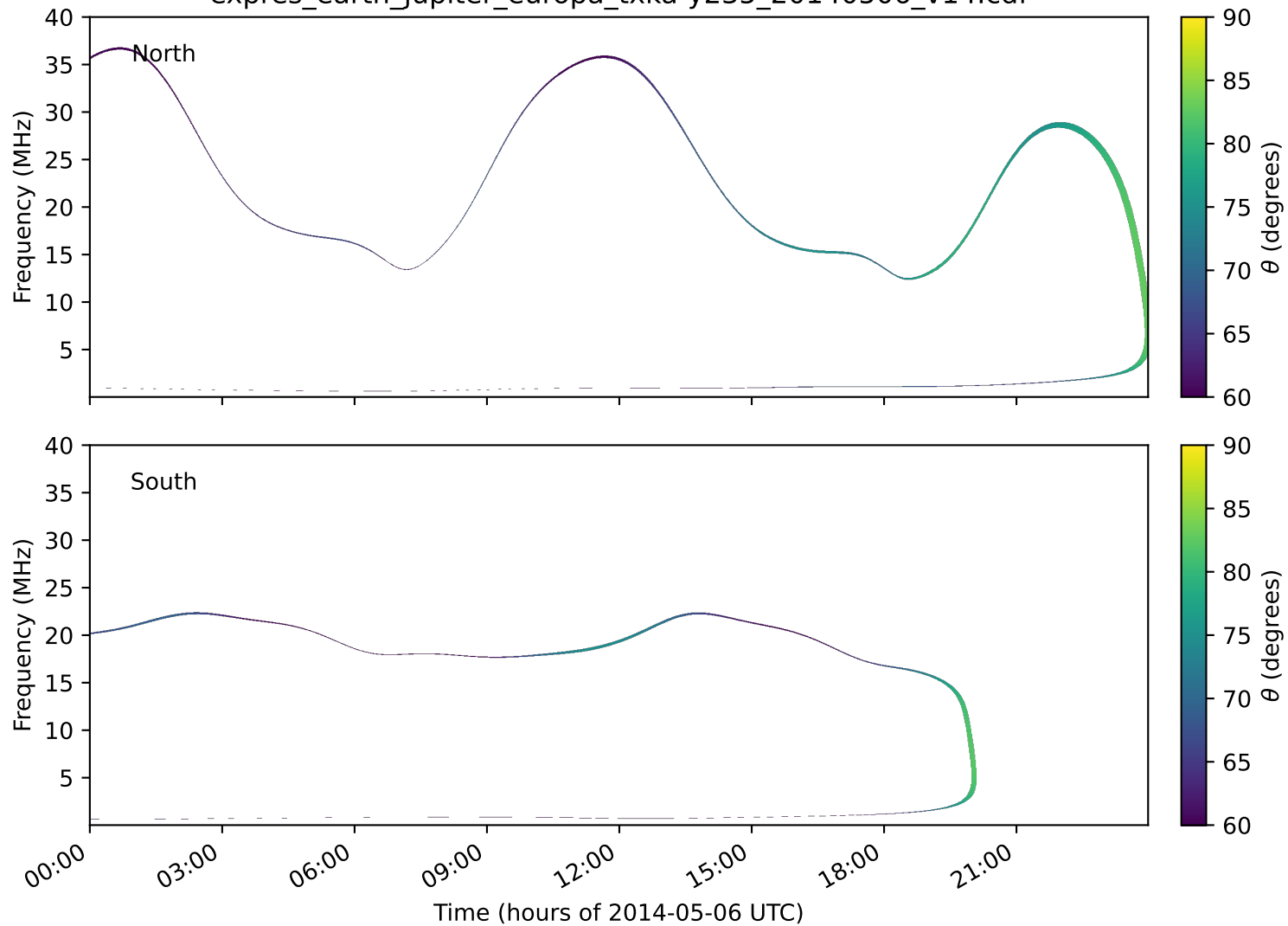
expres_earth_jupiter_europa_txka-y235_20140506_v14.cdf
