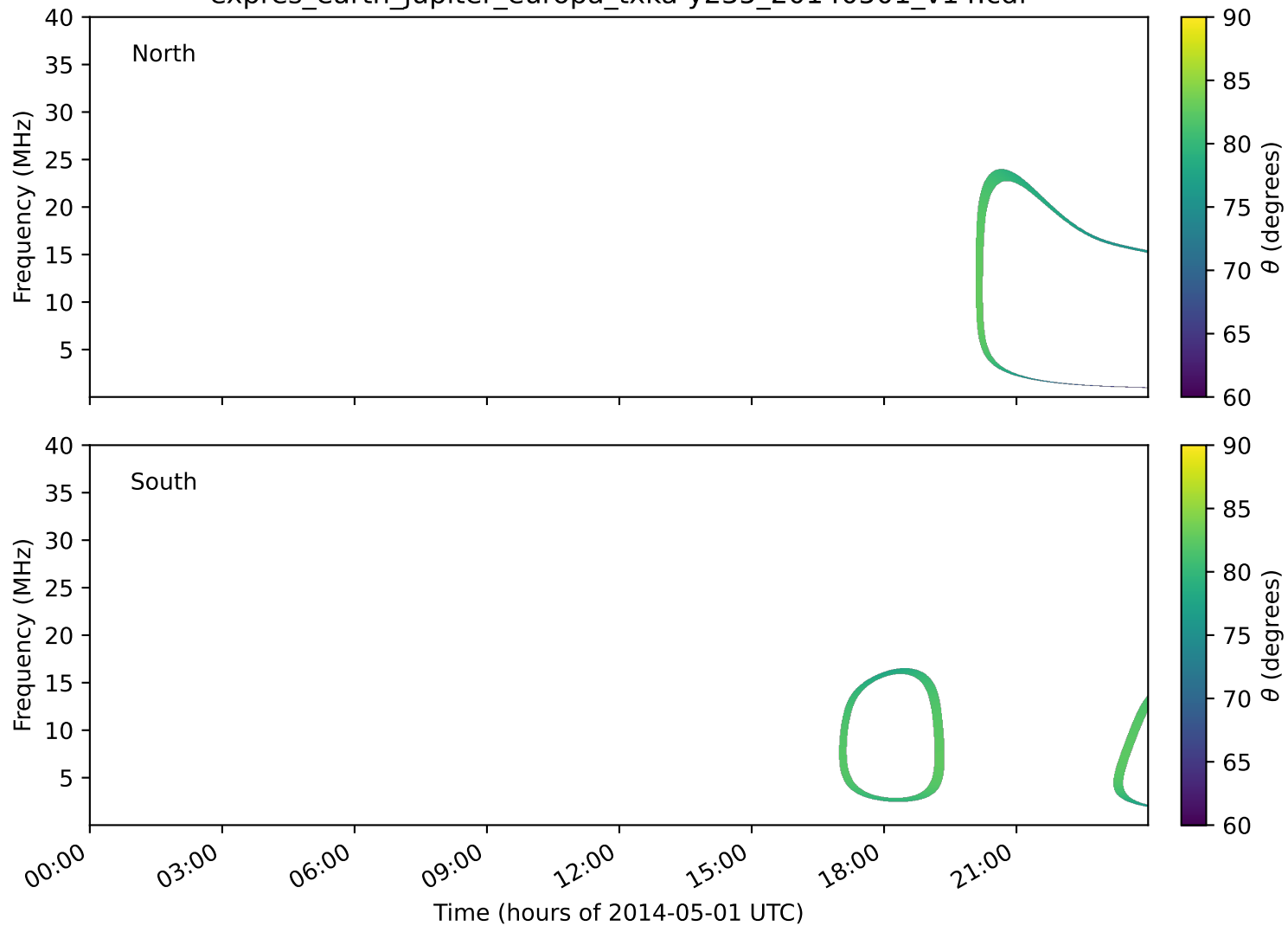
expres_earth_jupiter_europa_txka-y235_20140501_v14.cdf
