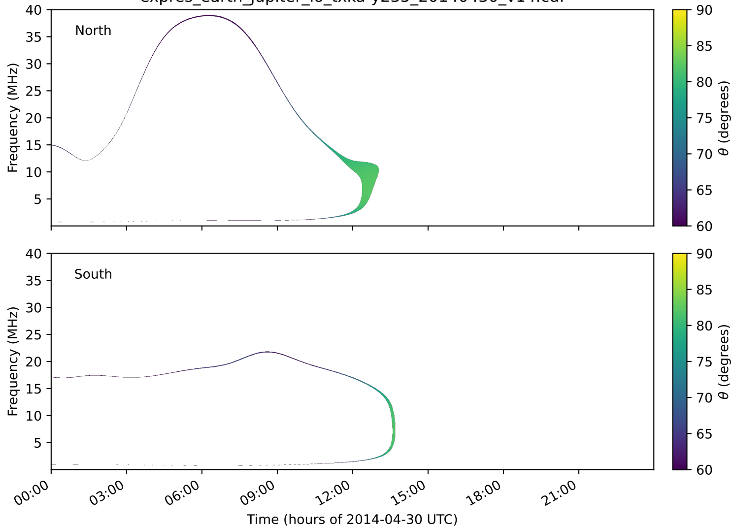
expres_earth_jupiter_io_txka-y235_20140430_v14.cdf
