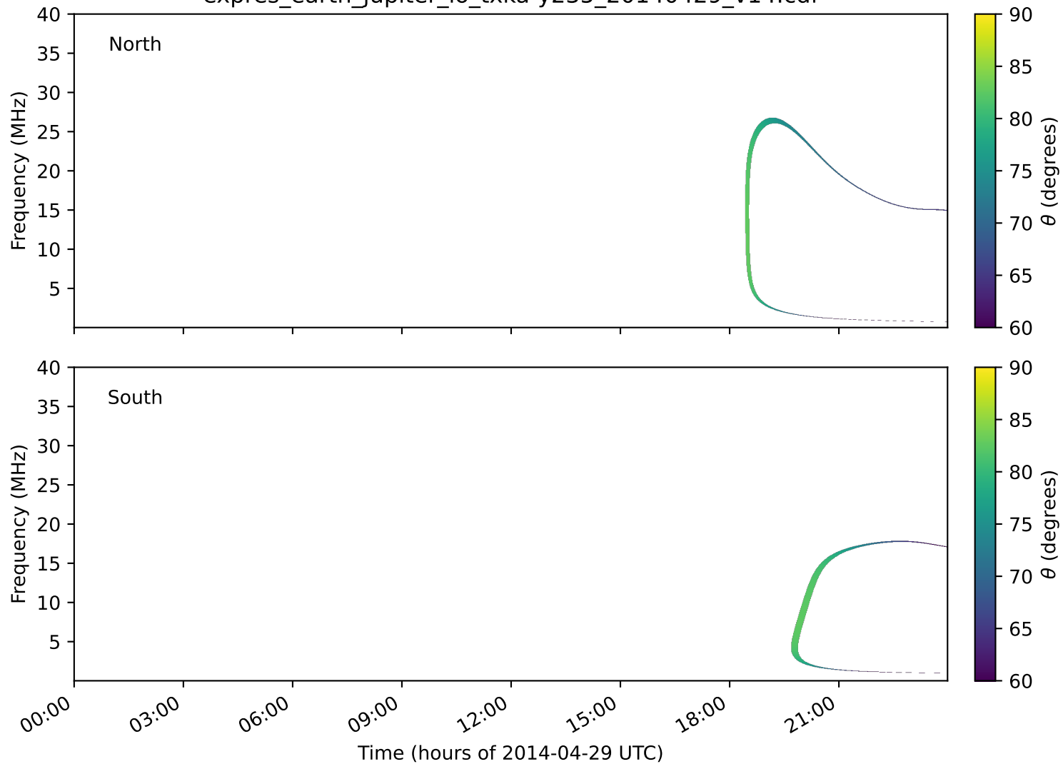
expres_earth_jupiter_io_txka-y235_20140429_v14.cdf
