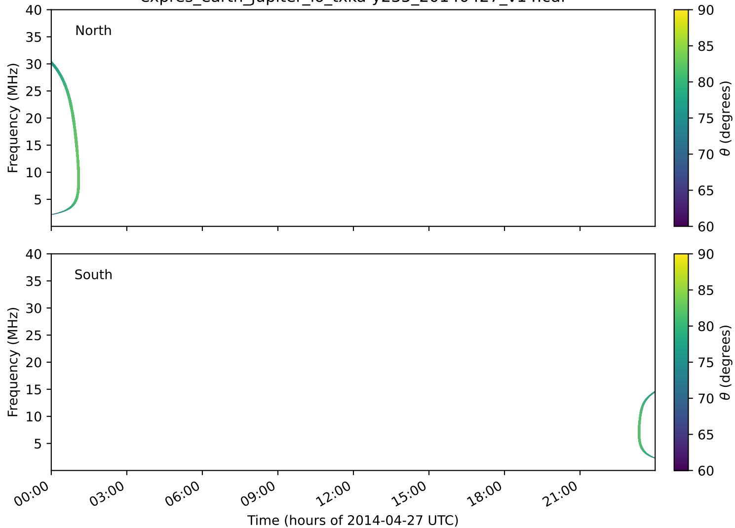
expres_earth_jupiter_io_txka-y235_20140427_v14.cdf
