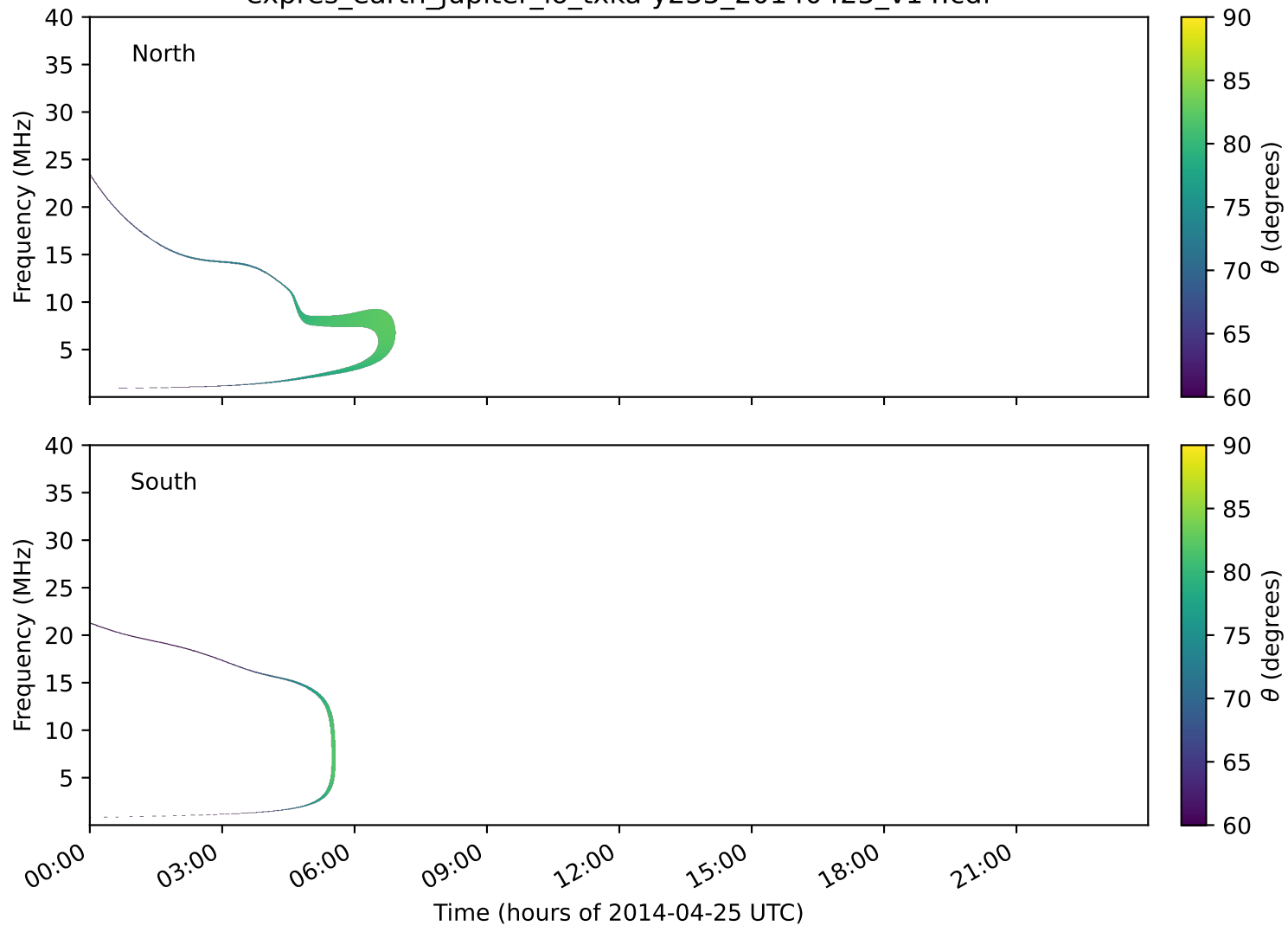
expres_earth_jupiter_io_txka-y235_20140425_v14.cdf
