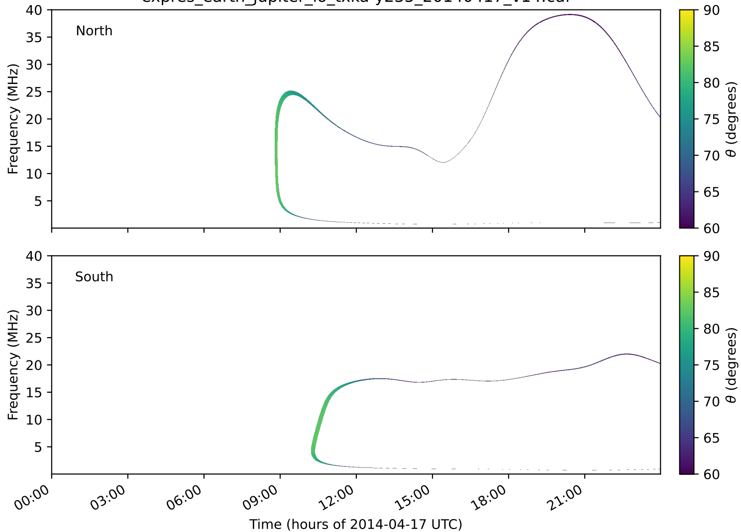
expres_earth_jupiter_io_txka-y235_20140417_v14.cdf
