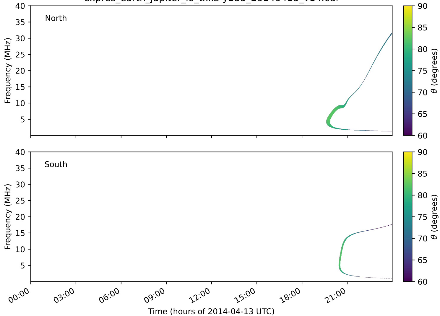
expres_earth_jupiter_io_txka-y235_20140413_v14.cdf
