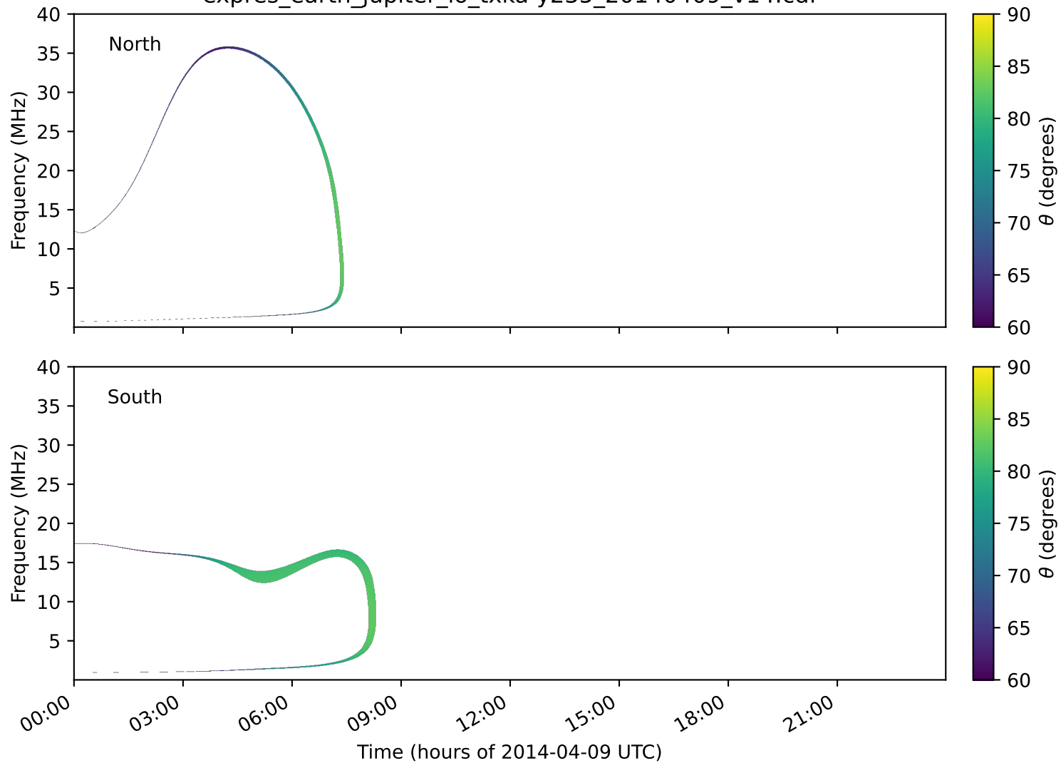
expres_earth_jupiter_io_txka-y235_20140409_v14.cdf
