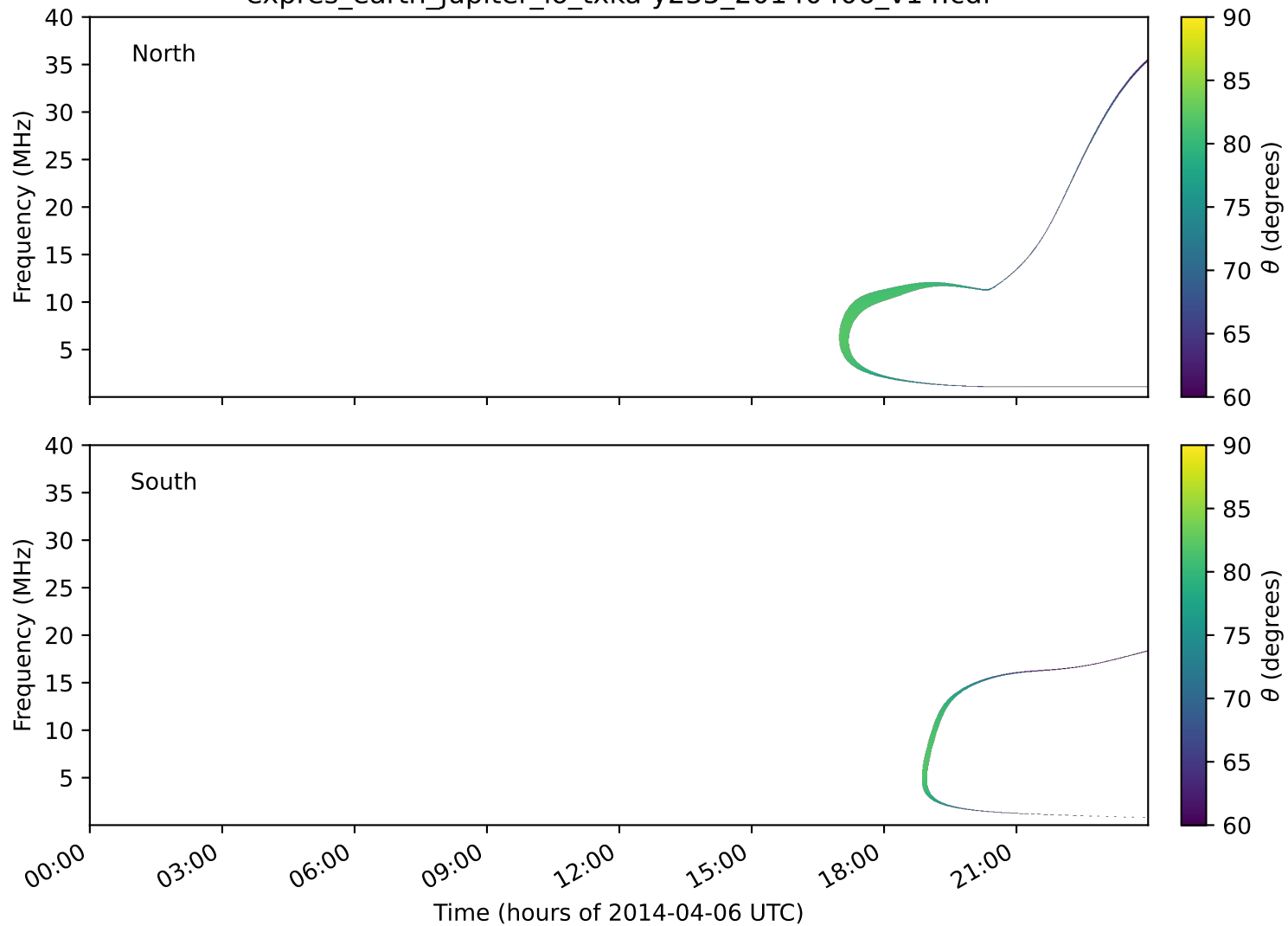
expres_earth_jupiter_io_txka-y235_20140406_v14.cdf
