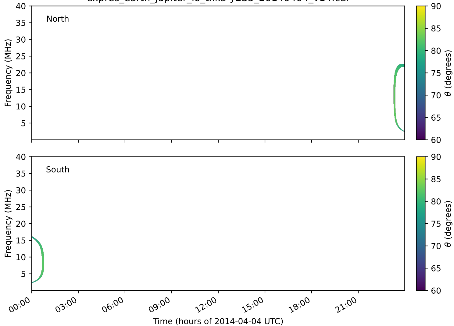
expres_earth_jupiter_io_txka-y235_20140404_v14.cdf
