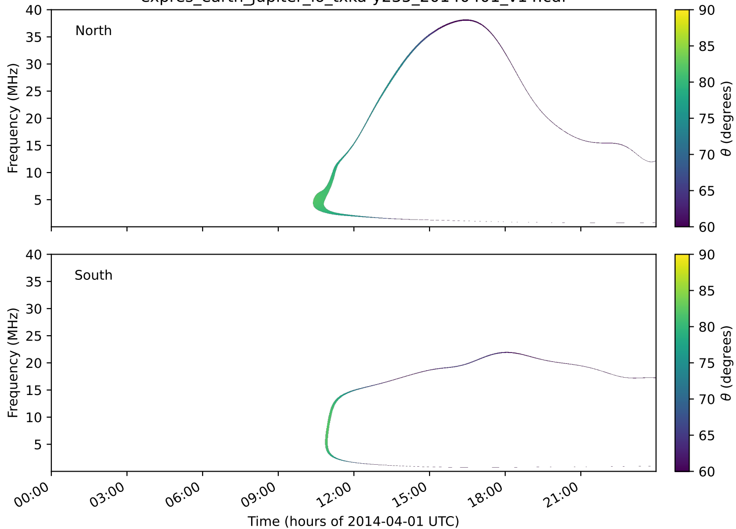
expres_earth_jupiter_io_txka-y235_20140401_v14.cdf
