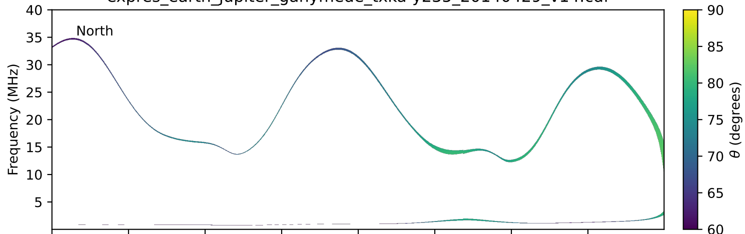
expres_earth_jupiter_ganymede_txka-y235_20140429_v14.cdf
