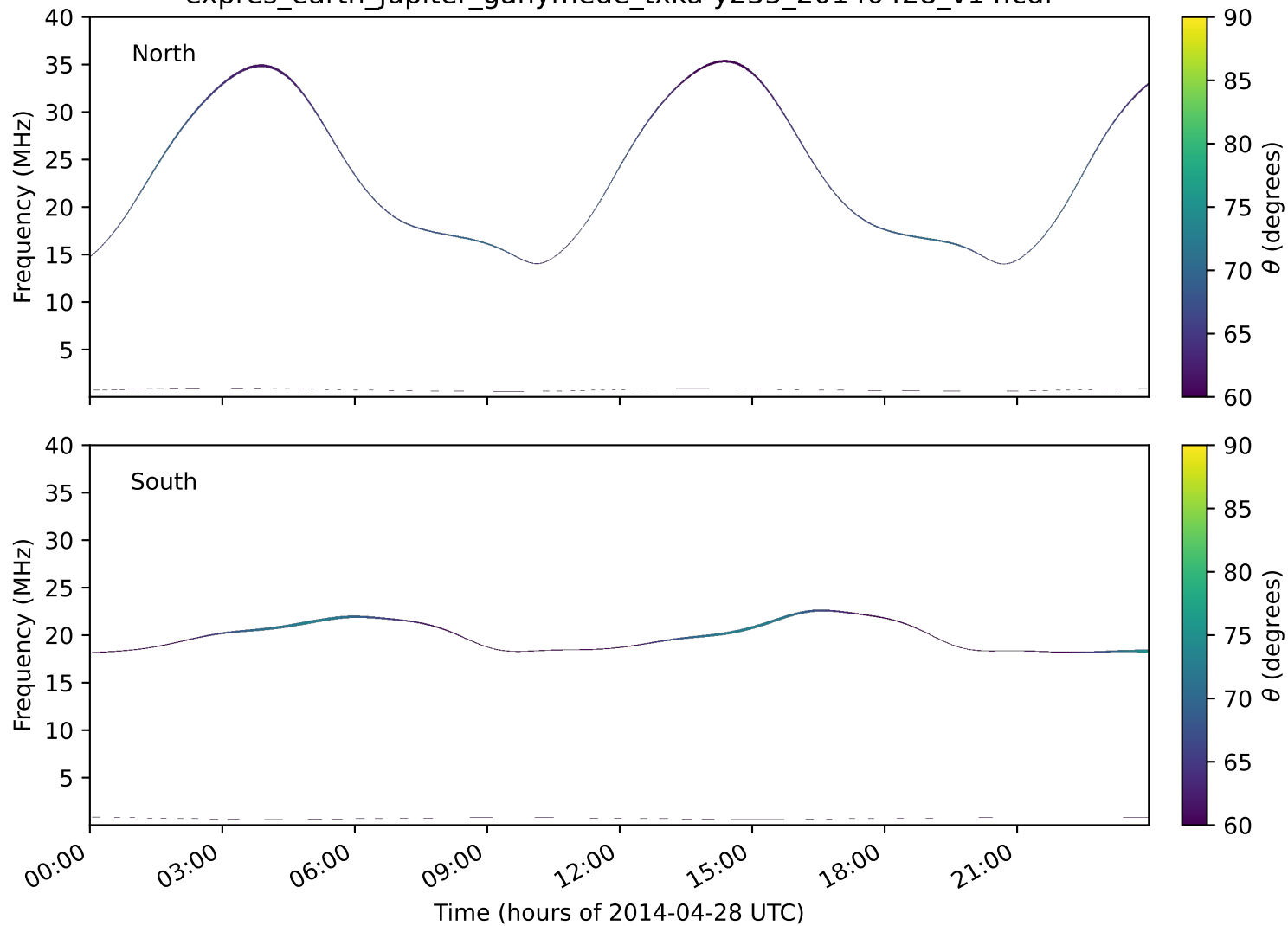
expres_earth_jupiter_ganymede_txka-y235_20140428_v14.cdf
