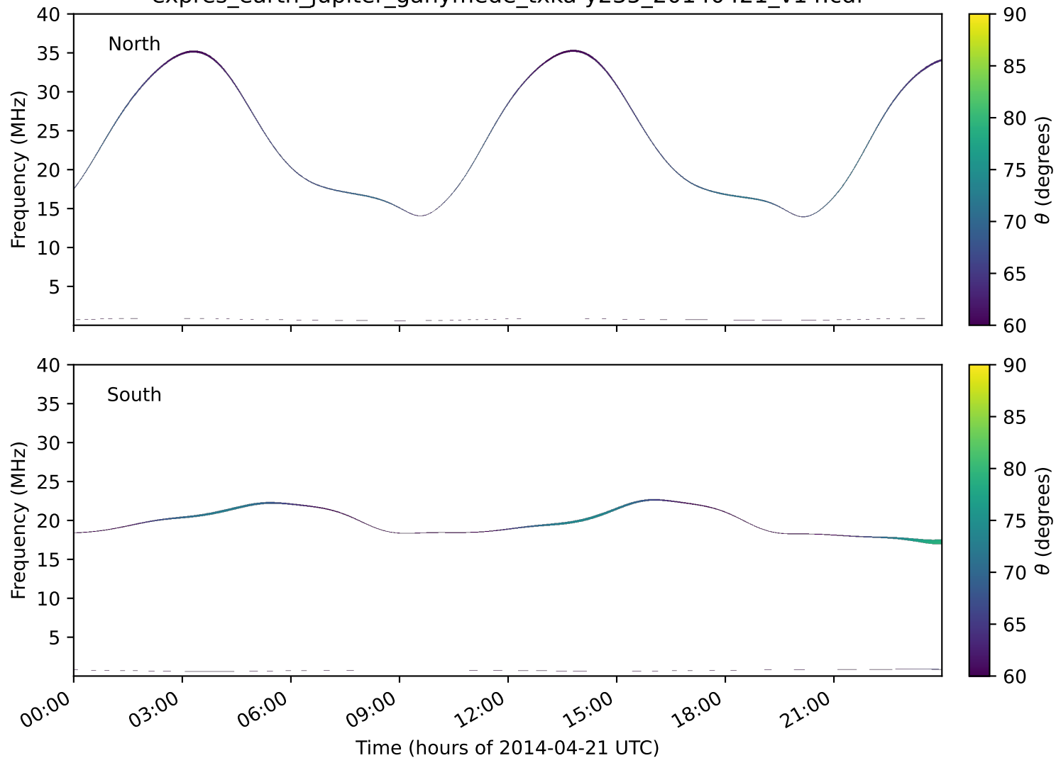
expres_earth_jupiter_ganymede_txka-y235_20140421_v14.cdf
