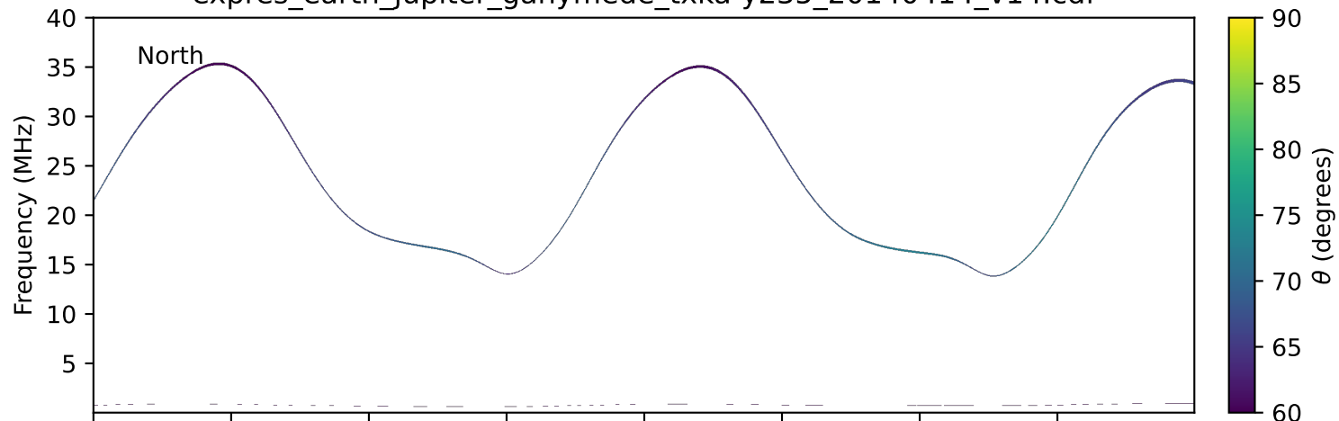
expres_earth_jupiter_ganymede_txka-y235_20140414_v14.cdf
