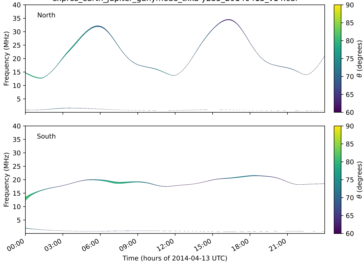
expres_earth_jupiter_ganymede_txka-y235_20140413_v14.cdf
