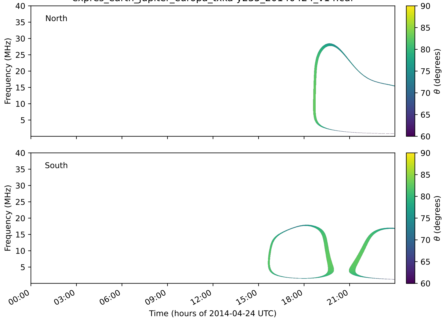
expres_earth_jupiter_europa_txka-y235_20140424_v14.cdf
