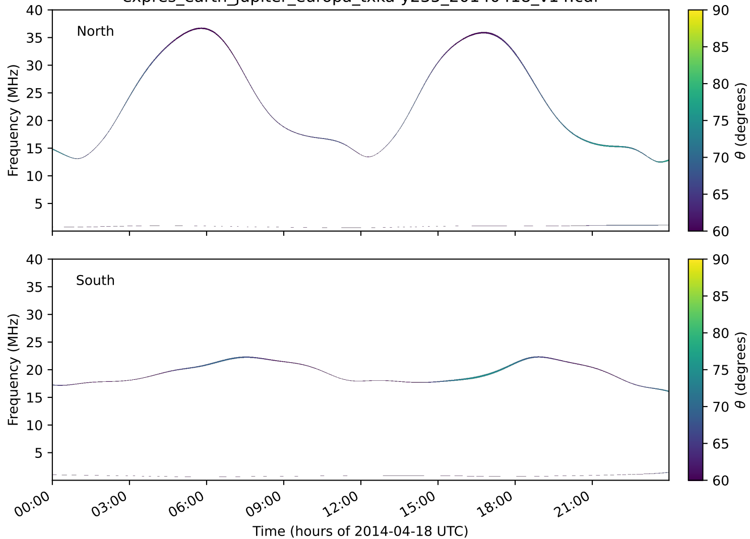
expres_earth_jupiter_europa_txka-y235_20140418_v14.cdf
