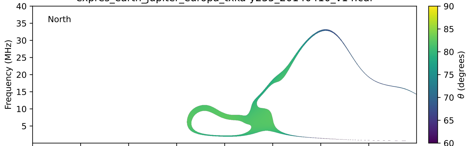
expres_earth_jupiter_europa_txka-y235_20140410_v14.cdf
