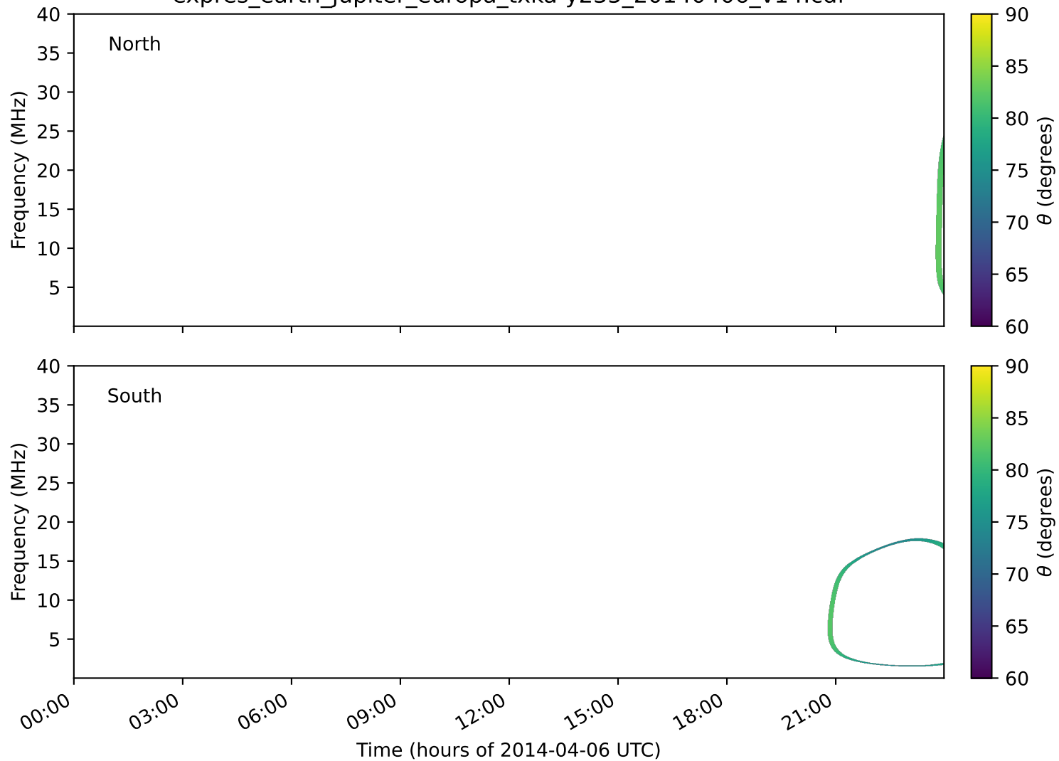
expres_earth_jupiter_europa_txka-y235_20140406_v14.cdf
