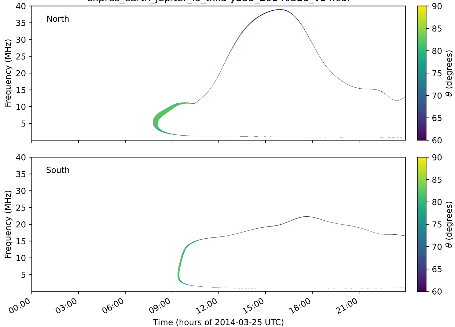
expres_earth_jupiter_io_txka-y235_20140325_v14.cdf
