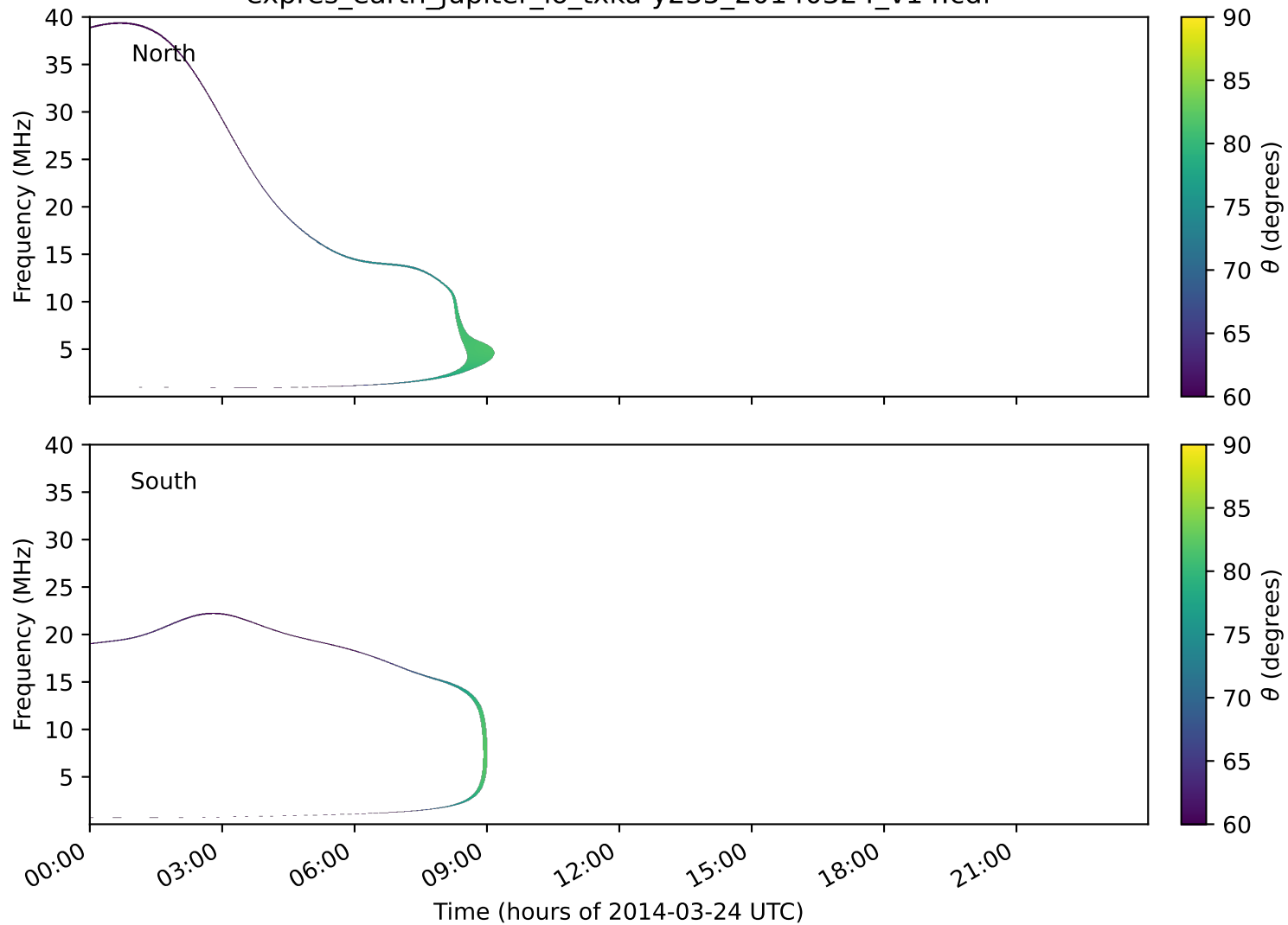
expres_earth_jupiter_io_txka-y235_20140324_v14.cdf
