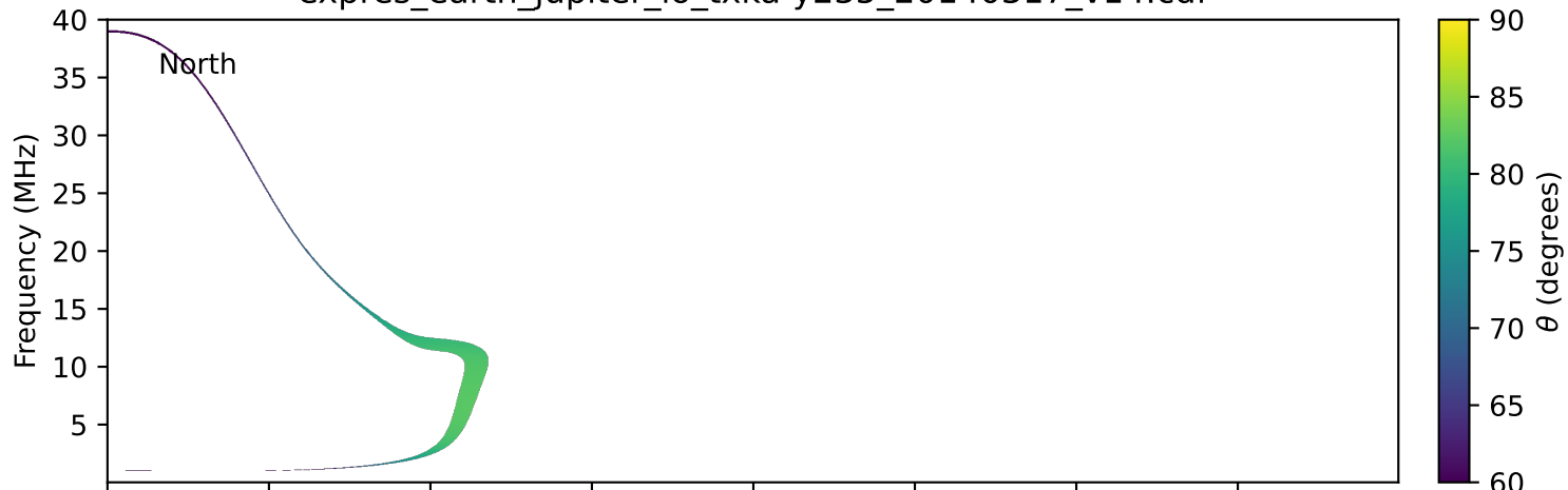
expres_earth_jupiter_io_txka-y235_20140317_v14.cdf
