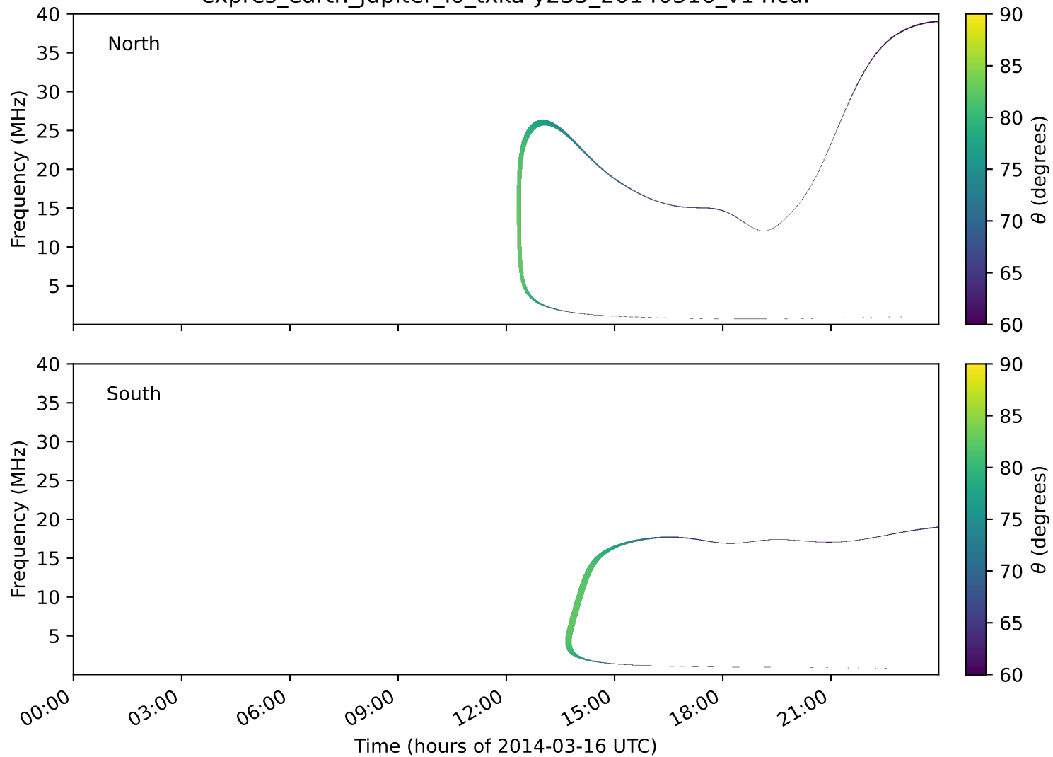
expres_earth_jupiter_io_txka-y235_20140316_v14.cdf
