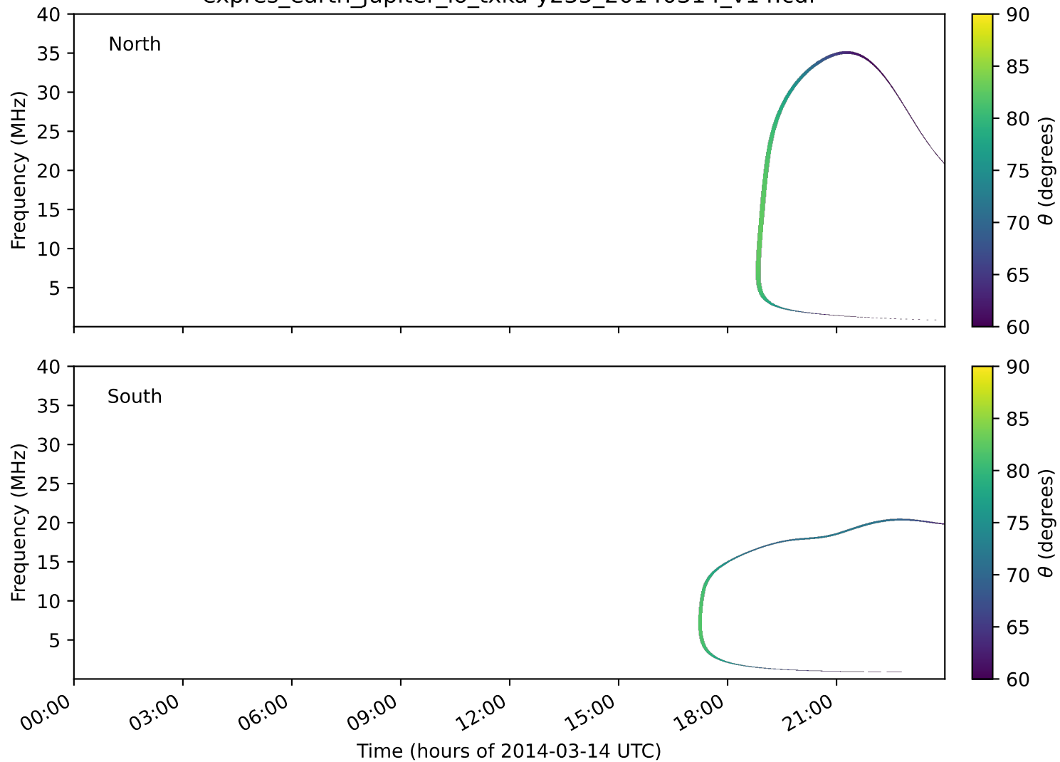
expres_earth_jupiter_io_txka-y235_20140314_v14.cdf
