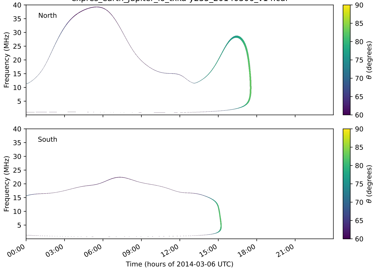
expres_earth_jupiter_io_txka-y235_20140306_v14.cdf
