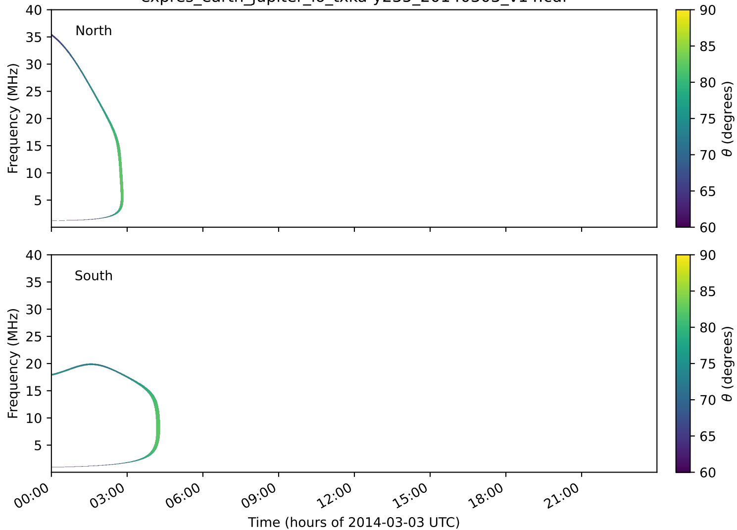
expres_earth_jupiter_io_txka-y235_20140303_v14.cdf
