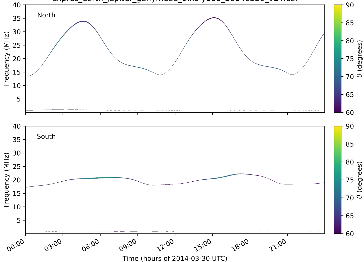
expres_earth_jupiter_ganymede_txka-y235_20140330_v14.cdf
