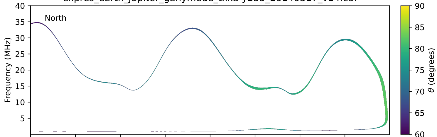
expres_earth_jupiter_ganymede_txka-y235_20140317_v14.cdf
