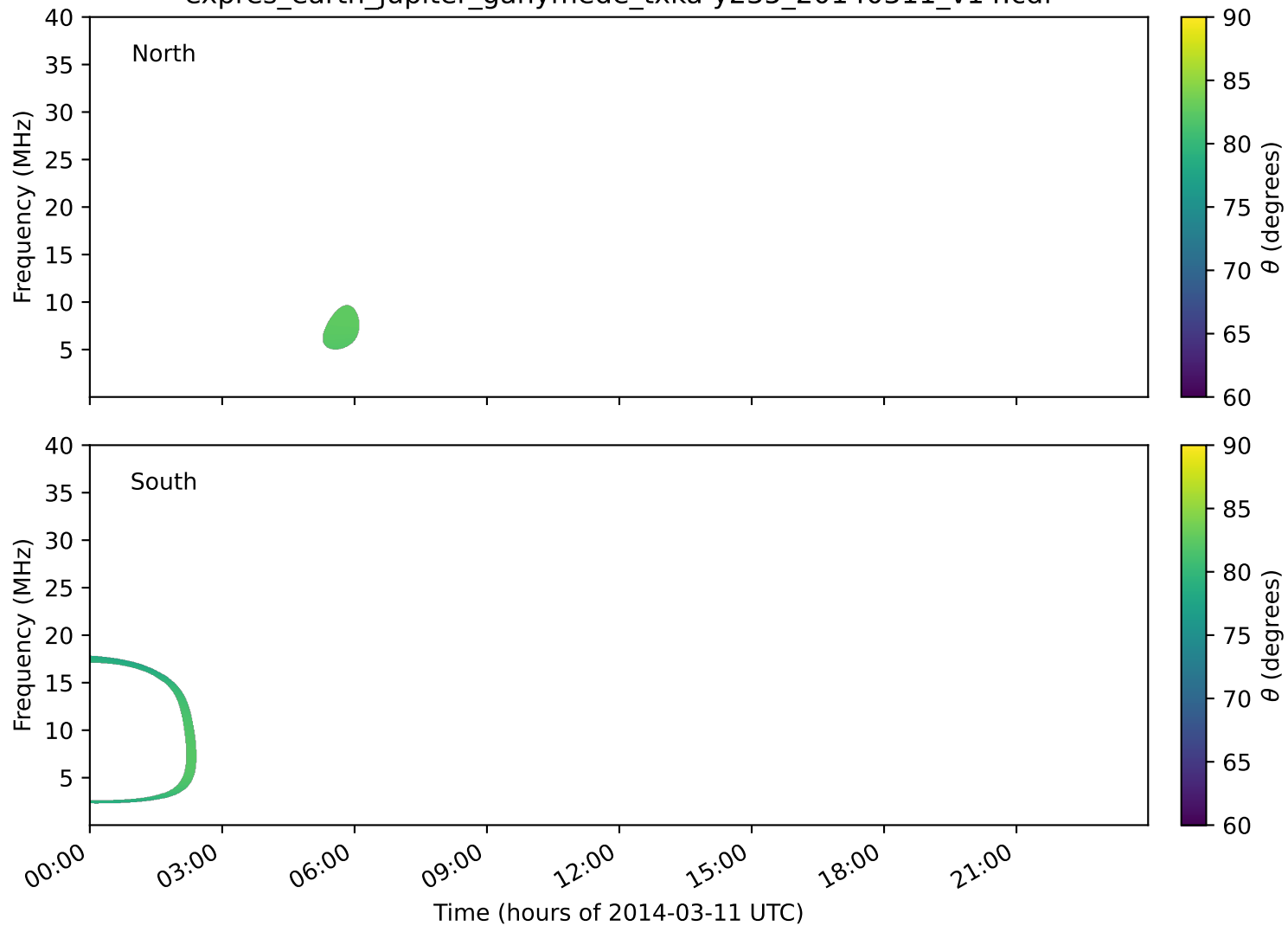
expres_earth_jupiter_ganymede_txka-y235_20140311_v14.cdf
