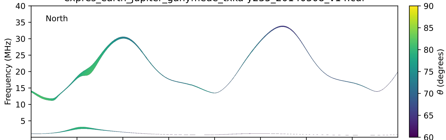
expres_earth_jupiter_ganymede_txka-y235_20140308_v14.cdf
