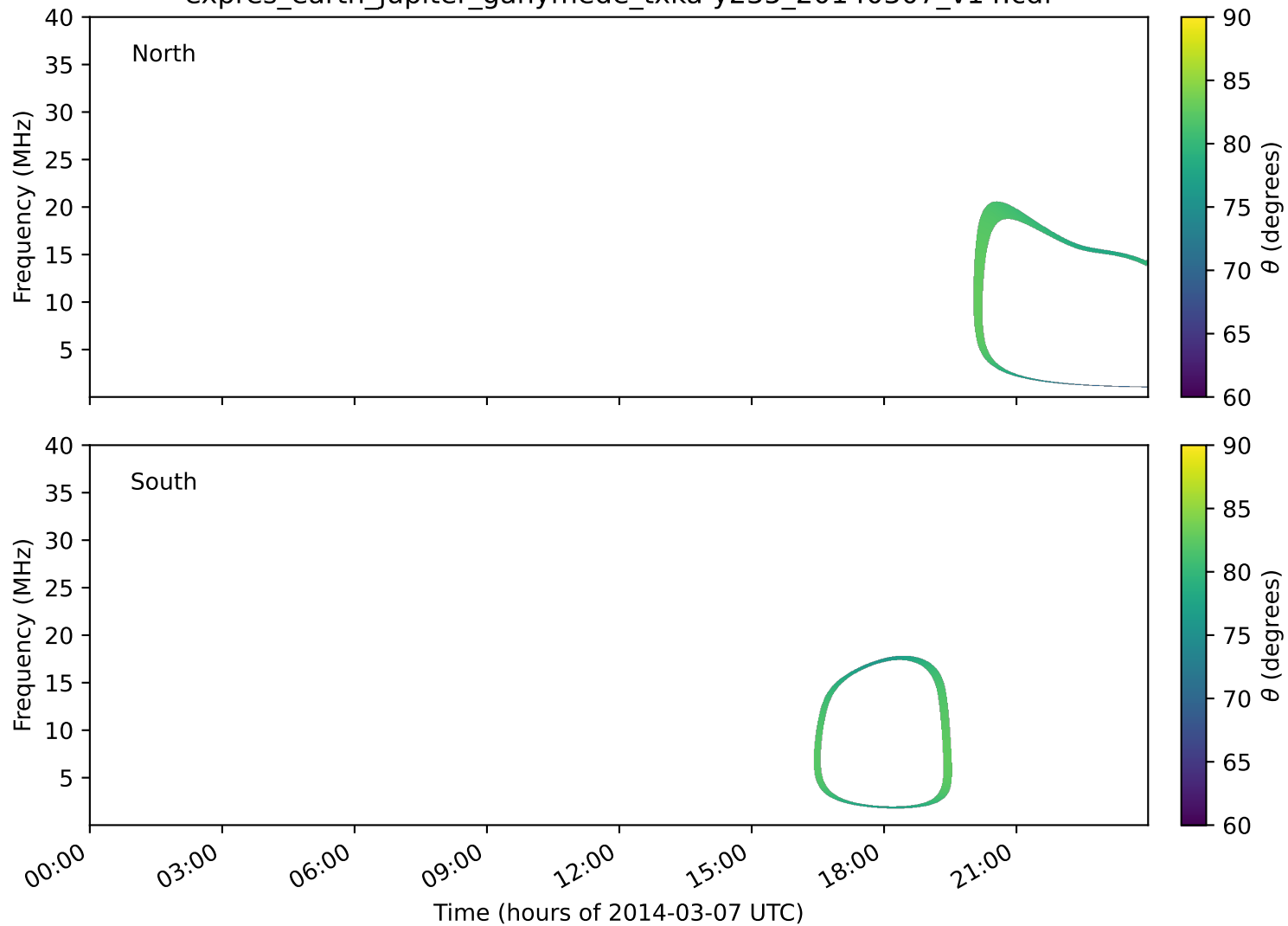
expres_earth_jupiter_ganymede_txka-y235_20140307_v14.cdf
