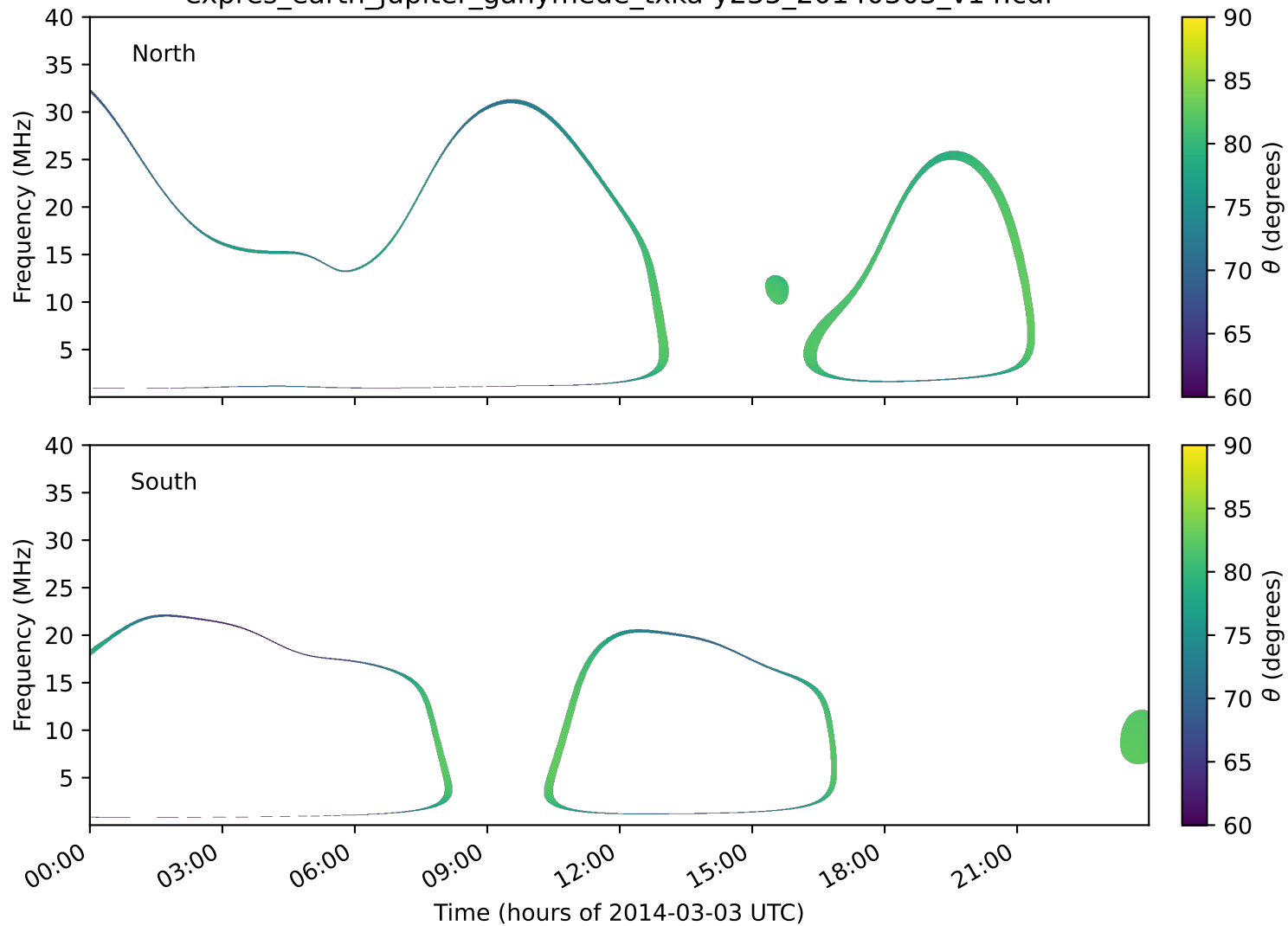
expres_earth_jupiter_ganymede_txka-y235_20140303_v14.cdf
