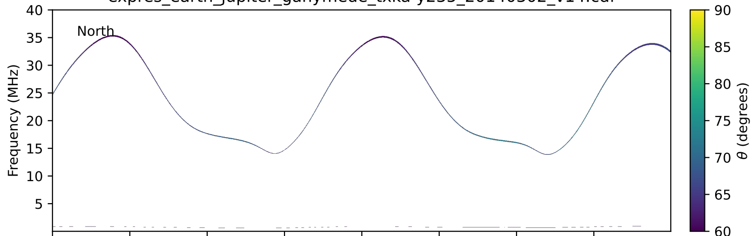
expres_earth_jupiter_ganymede_txka-y235_20140302_v14.cdf
