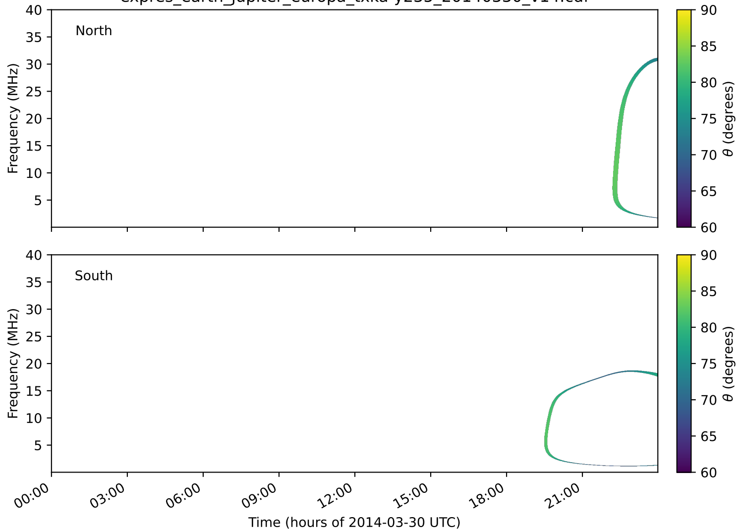
expres_earth_jupiter_europa_txka-y235_20140330_v14.cdf
