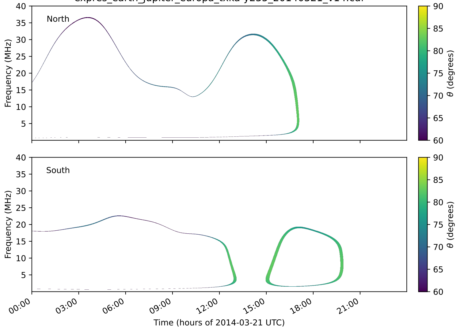
expres_earth_jupiter_europa_txka-y235_20140321_v14.cdf
