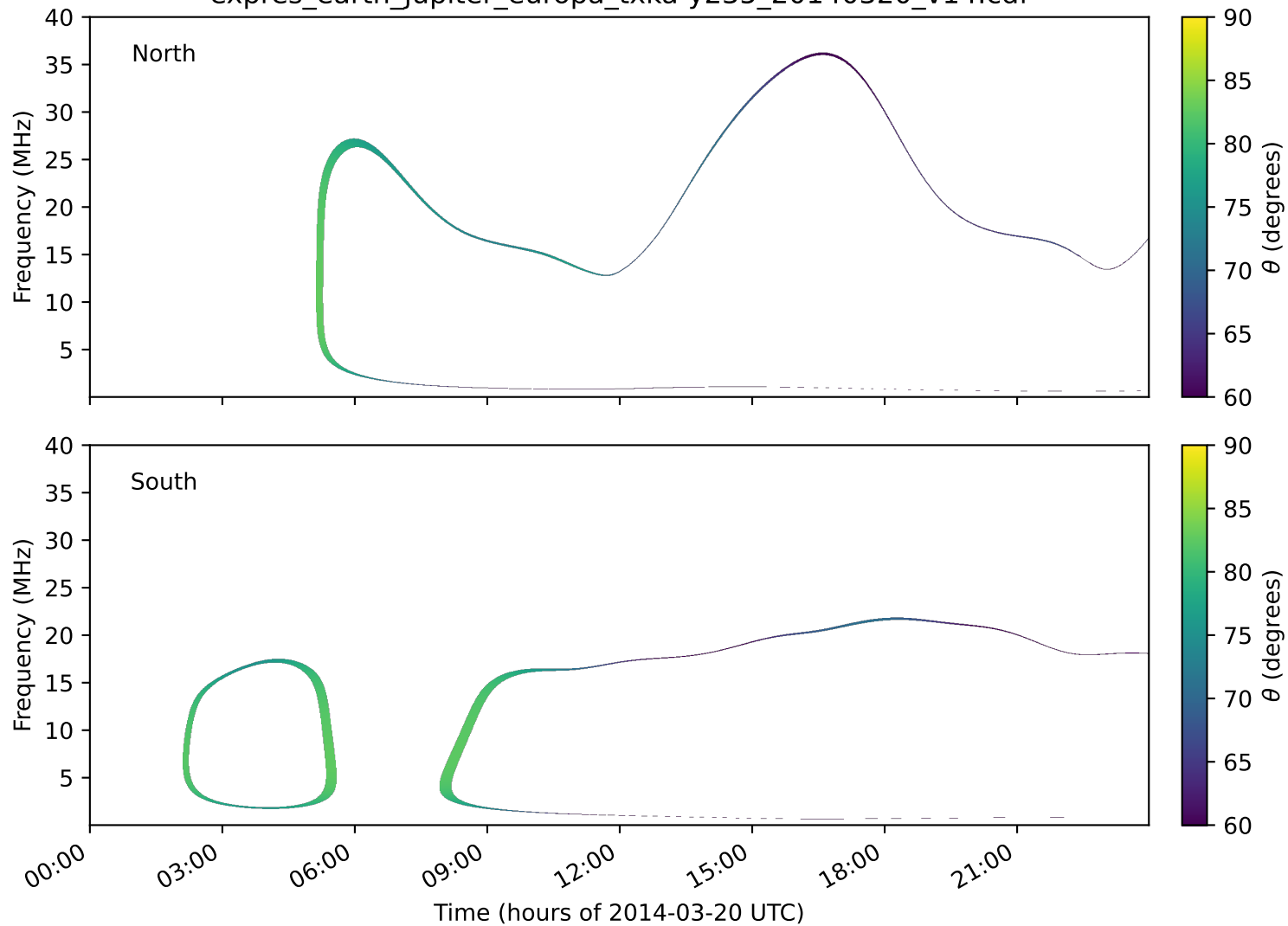
expres_earth_jupiter_europa_txka-y235_20140320_v14.cdf
