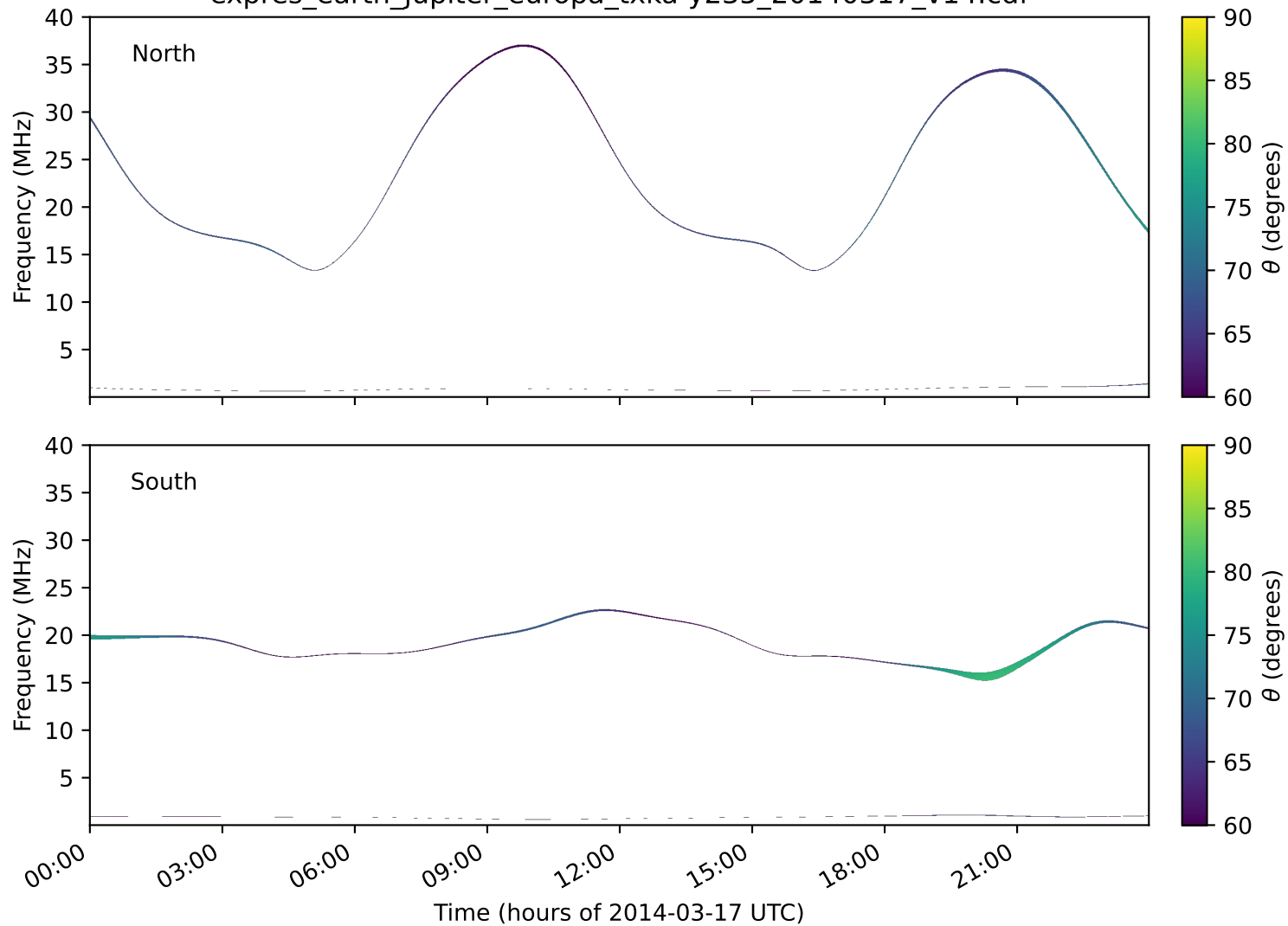
expres_earth_jupiter_europa_txka-y235_20140317_v14.cdf
