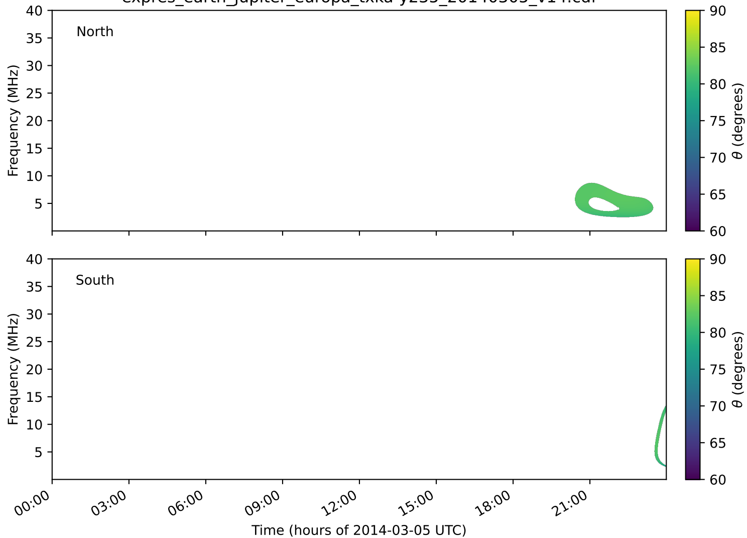
expres_earth_jupiter_europa_txka-y235_20140305_v14.cdf
