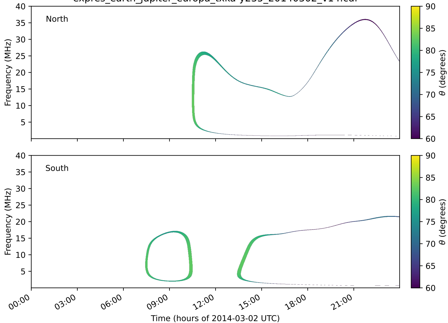
expres_earth_jupiter_europa_txka-y235_20140302_v14.cdf
